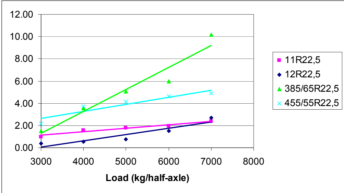
Figure 33 - N_{\text{Benkelman}}/N_{\text{trial}} ratio corresponding to the distortions at the pavement base in relation to load per half-axle at a pressure of 730 kPa (spring trials)
